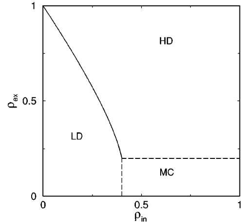
FIG. 4. Phase diagram for the ASEP with diffusive injection and extraction of particles, i.e., for the case C shown in Fig. 1. The parameters are v=0.1 , D=1/2 , and L_1=L_3=6 .
